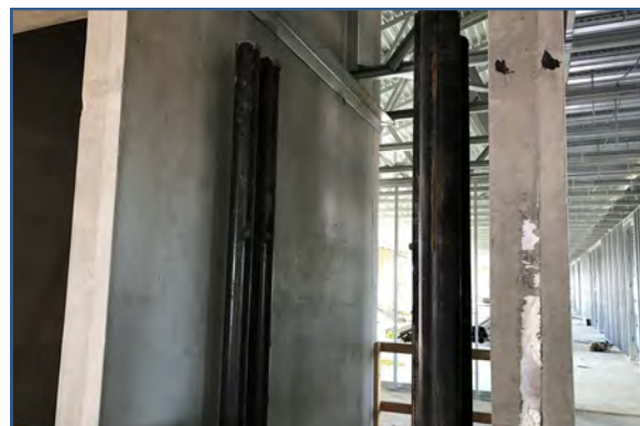
Bldg. B Supply & Return Chilled Water Piping
