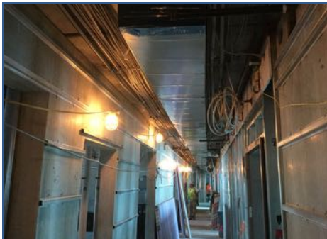
Bldg. A Overhead MEP Rough-In
